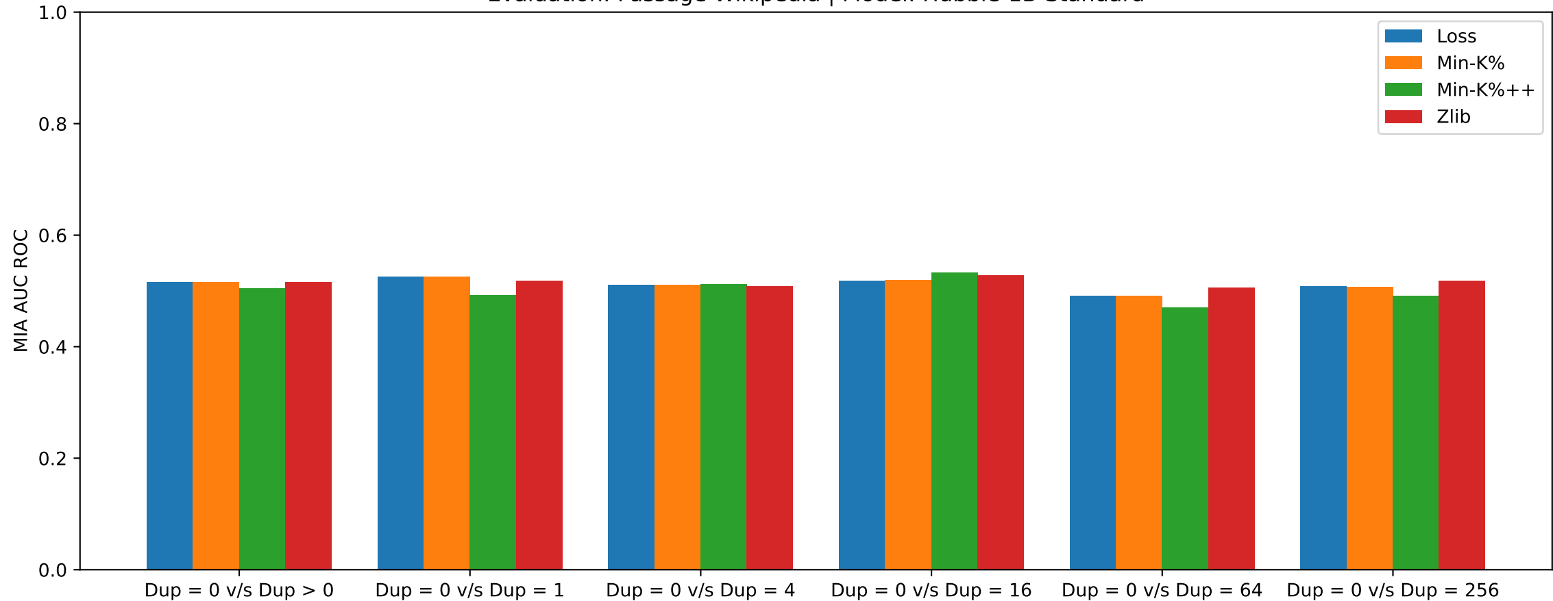
Evaluation: Passage Wikipedia | Model: Hubble-1B-Standard
